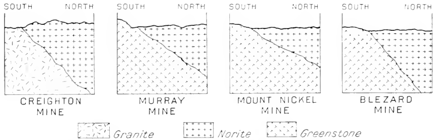
Fig. 8.—Cross-sections illustrating sill-like character of the basic edge of the norite-micropegmatite (the so-called nickel eruptive) on the southern nickel range, Sudbury, Ontario. These diagrams show that the norite-micropegmatite has partly a sill-like form.
